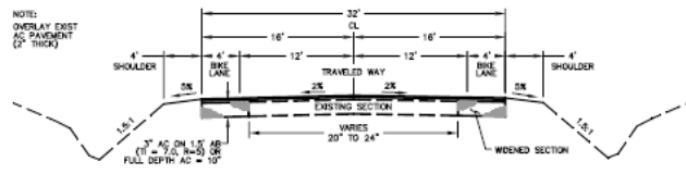
PITT SCHOOL RD. TYPICAL SECTION
